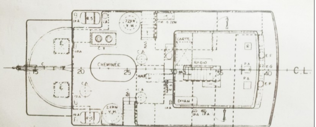
PASSERELLE DE NAVIGATION BRIDGE DECK
